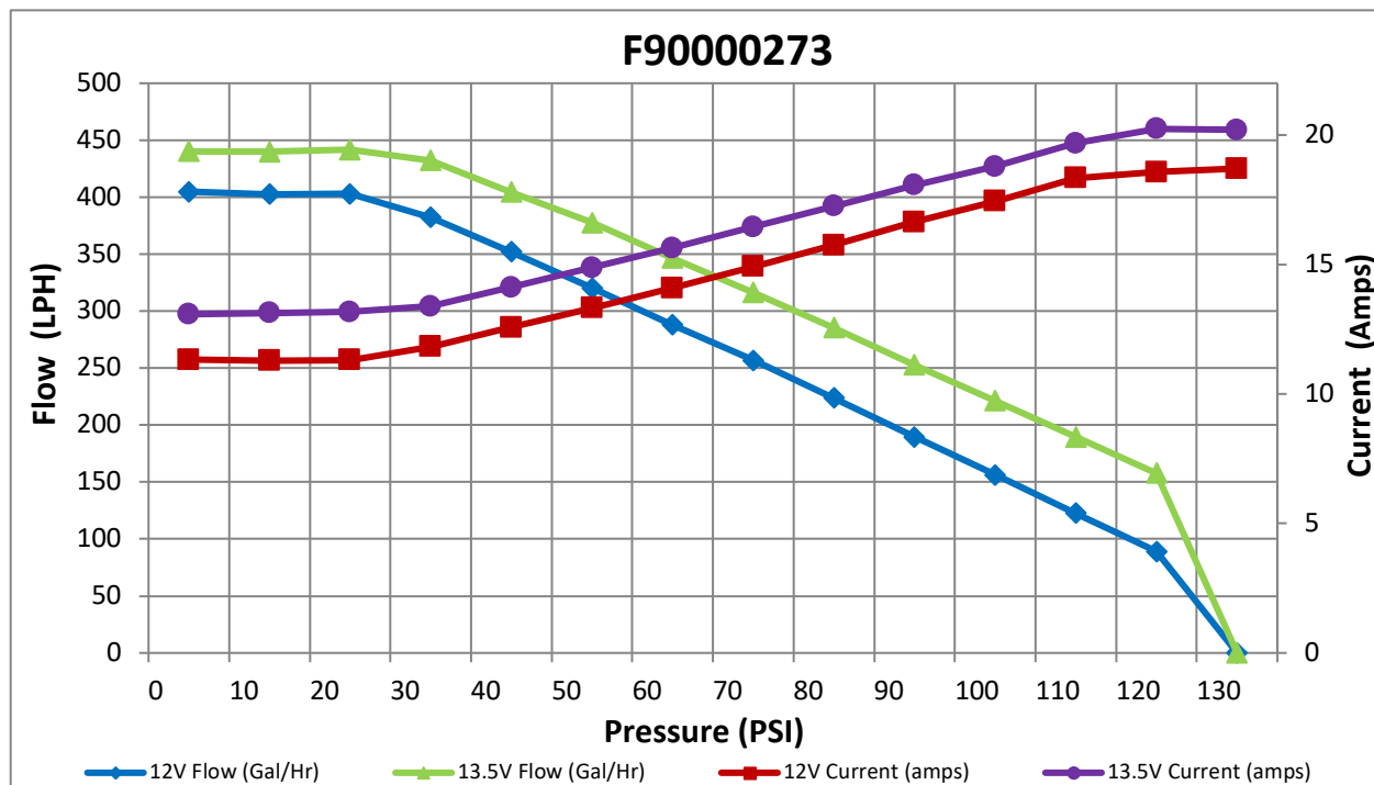
F90000273: 400LPH Gas Pump
